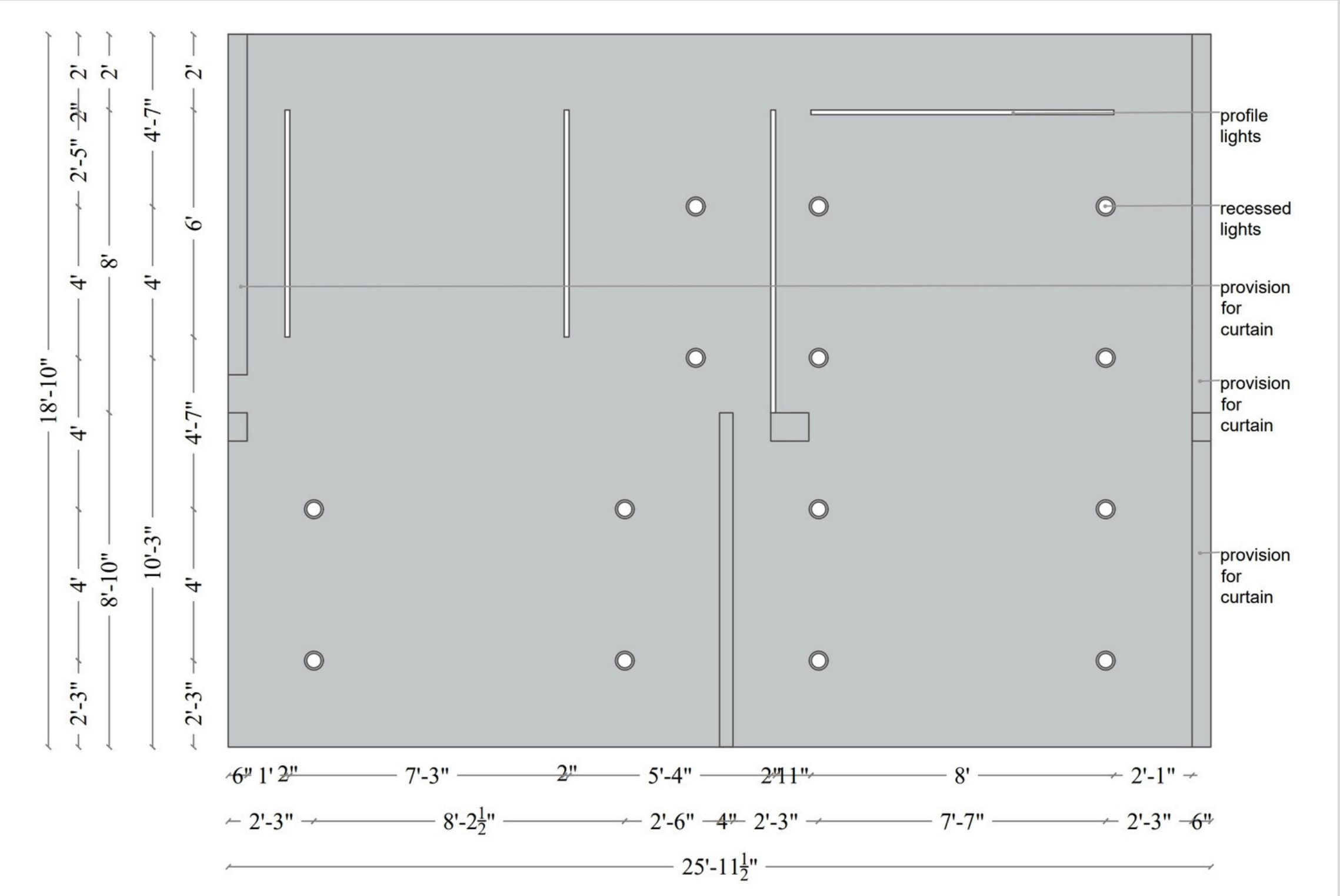
Ceiling Layout
